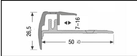
PF 320 Treppenkantenschiene 7-16 mm
