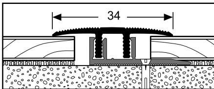
Clic transition profile 6 - 10 / 15 / 20 mm
