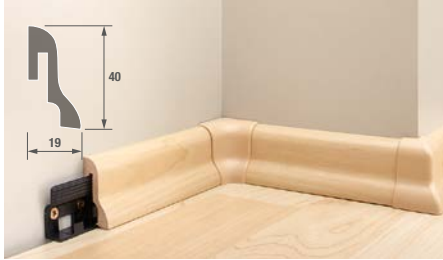
Base skirting SL 40
