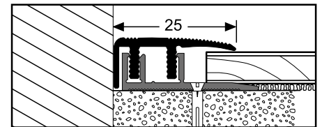
Click end profile 6 - 10 / 15 / 20 mm
