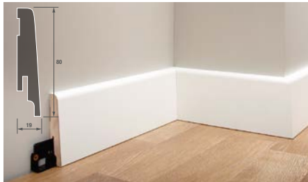
Decorative skirting AFL 80
