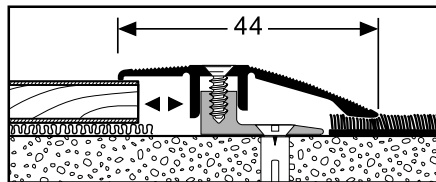
Screw-in joining profile 6.5 - 16 / 26 mm
