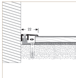
Screw-in End Profile 6,5 – 16 mm (26 mm with Lift up Block)
