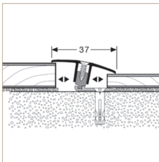
Screw-in Transition Profile with compensating till 5 mm at the same level 7–17 mm (27 mm with Lift up Block) at a different level 3–22 mm (32 mm with Lift up Block)
