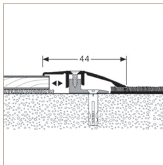
Screw-in Adapter Profile 6,5 – 16 mm (26 mm with Lift up Block)
