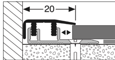
Clic-End Profile
