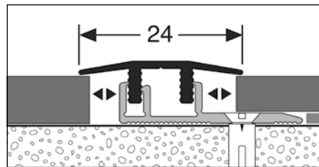
Clic-Transition Profile
