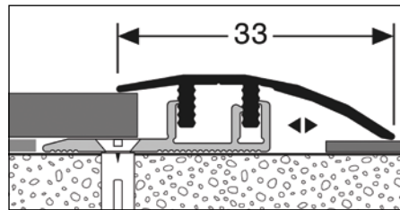
Clic-Adapter Profile
