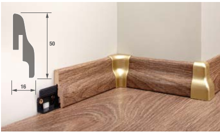
Clip-on skirting SFL 50 16 x 50 x 2700 mm
