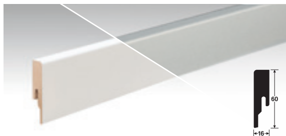
Accent skirting board ASL 60 (white, identical decor, stainless steel, anthracite, black) 16 x 60 x 2380 mm
