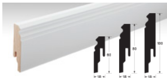
Hamburg skirting board HSL 60 | 80 | 100 (white) 18 x 60 x 2380 mm 18 x 80 x 2380 mm 18 x 100 x 2380 mm
