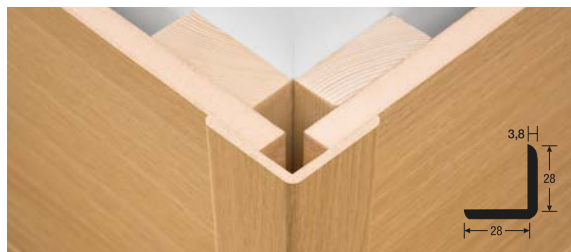
Corner moulding WKL 28/28
